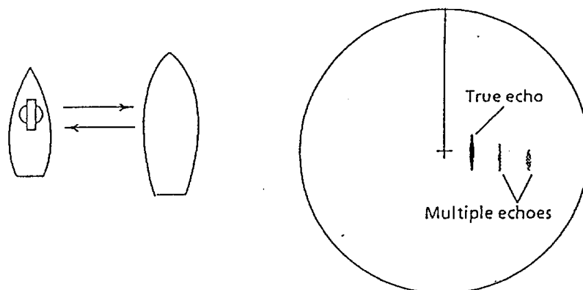
Figure 2-4 Multiple Echoes
