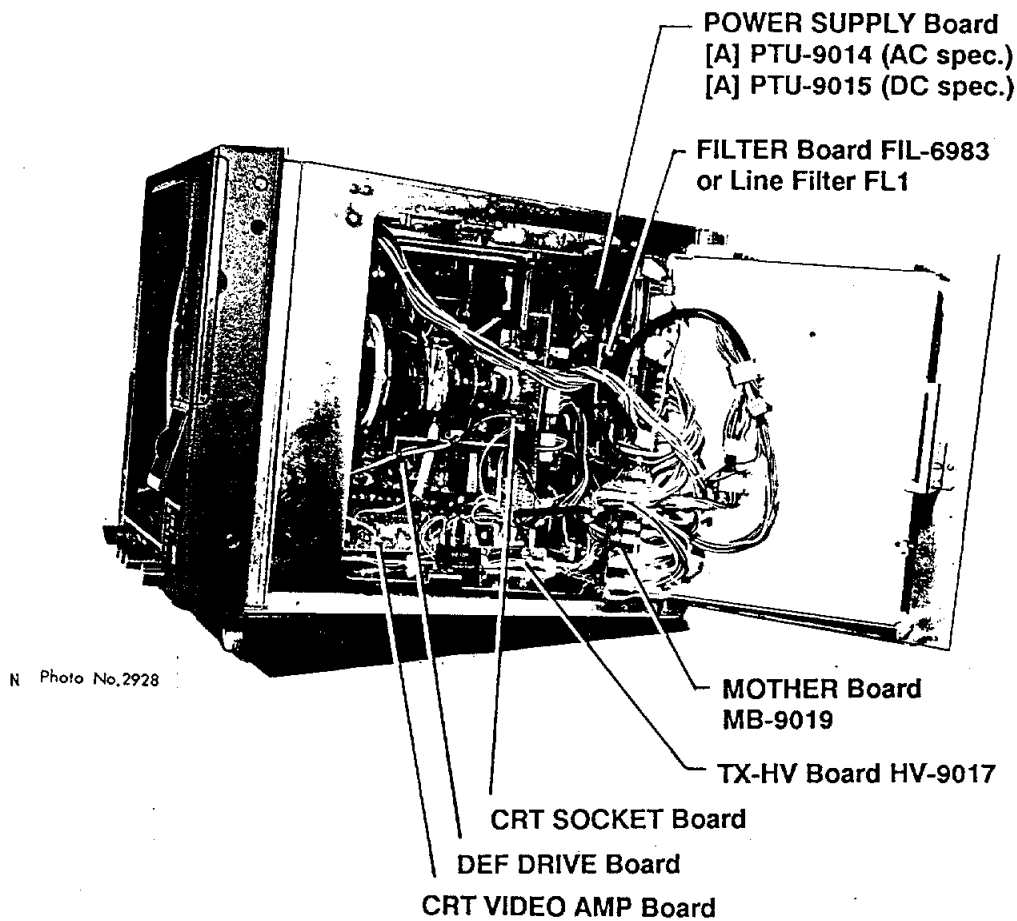
Figure 5-3 Display Unit, cover opened, right side view
