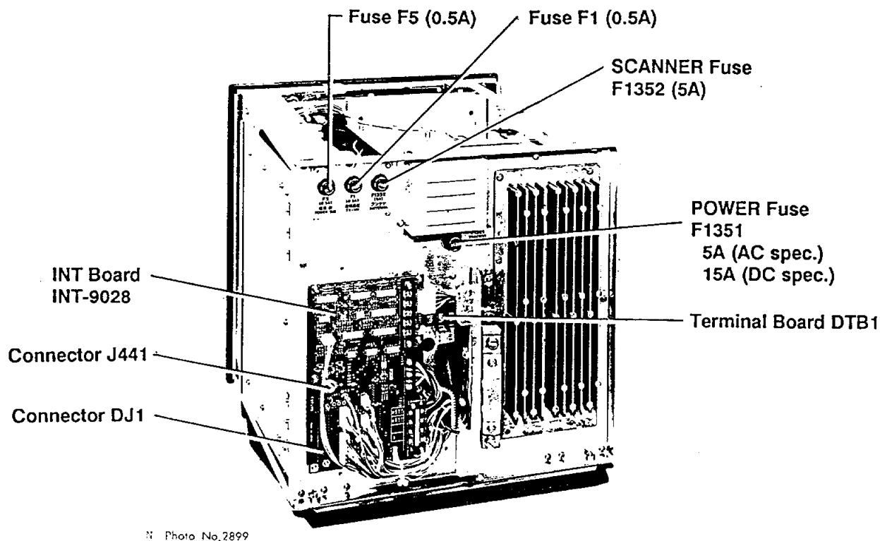
Figure 5-6 Display Unit, cover opened, rear view
