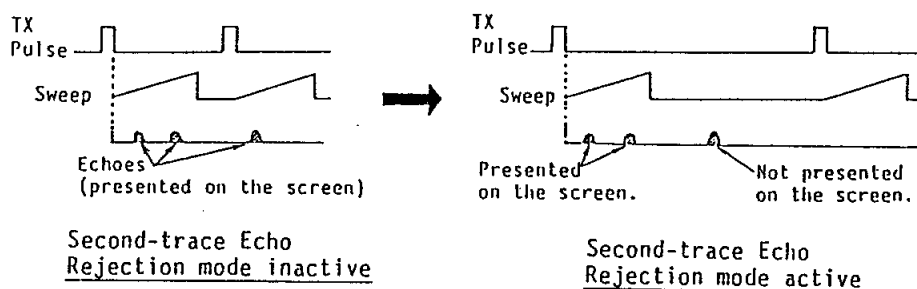
Figure 1-18 How the Second Trace Echo Rejection Circuit Works
