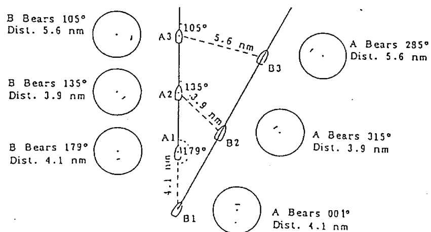
Figure 2-12 Relative Motion Versus True Motion
