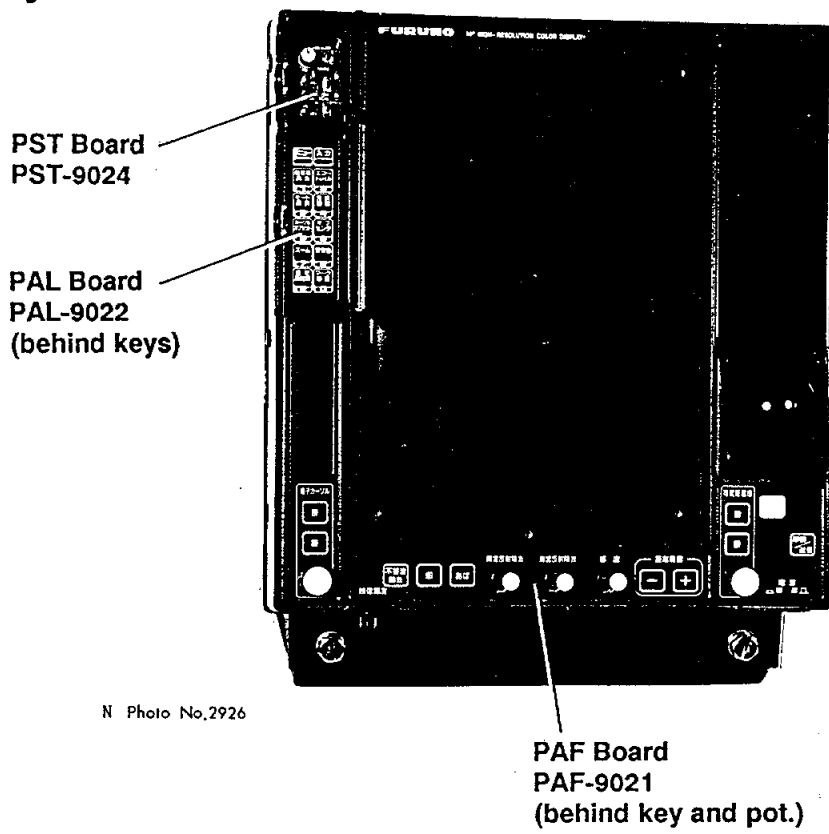
Figure 5-1 Display Unit, front view
