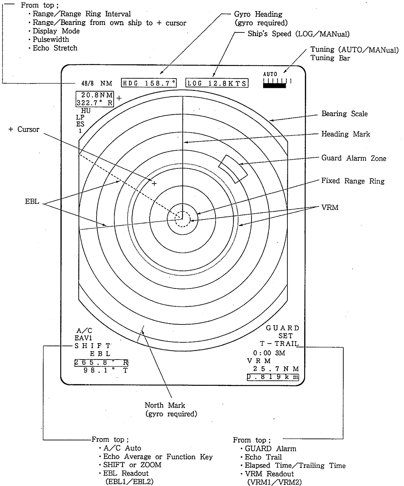
Figure 1-25 Markers and Indications
