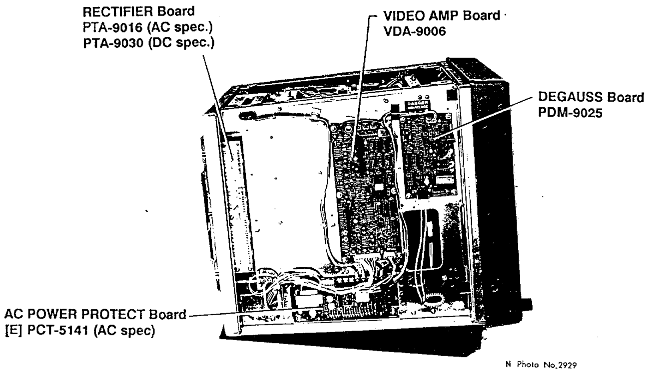
Figure 5-3 Display Unit, cover opened, right side view
