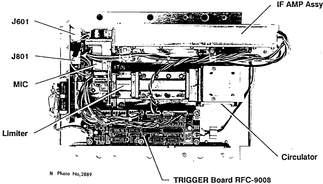
Figure 5-7 Transceiver Module
