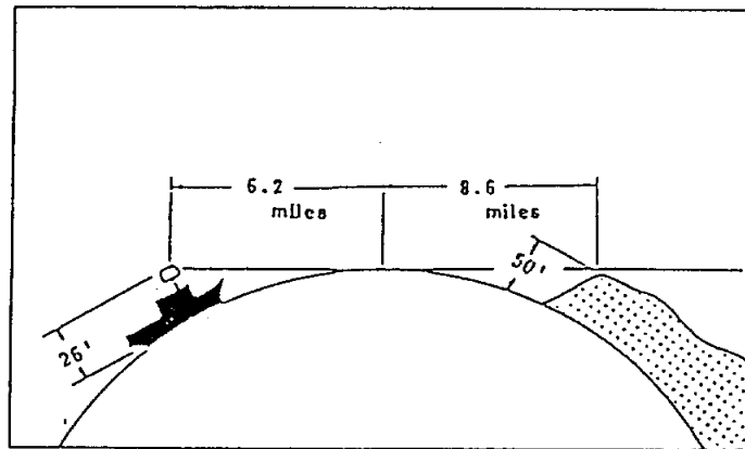
Figure 2-2 Radar Horizon
